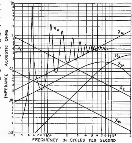
Fig. 3—Acoustic impedance characteristics of the system depicted in Fig. 1. R_H = acoustic resistance at the throat of the horn.
